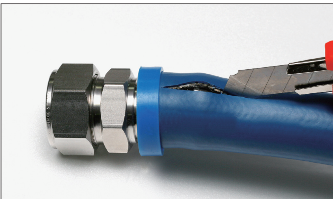
1. Slit hose lengthwise from blue finishing cap to end of barb. Do not damage barbs.
