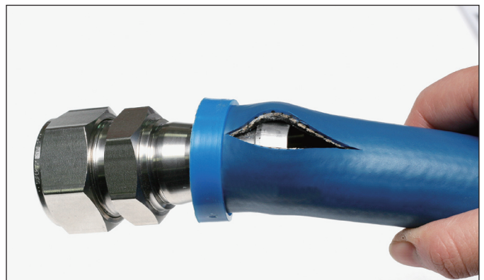
2. Bend hose to expose barbs, then remove hose with a quick pull.
