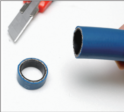
1. Cut a clean, square edge on end of hose
